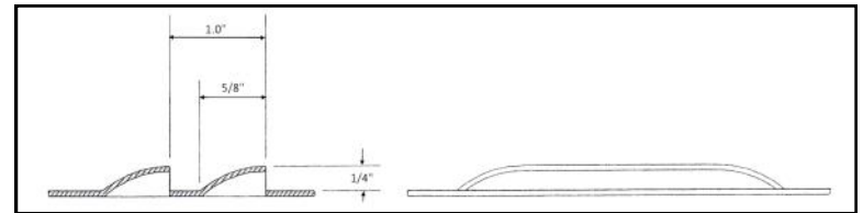
Detail of Louver Profile
